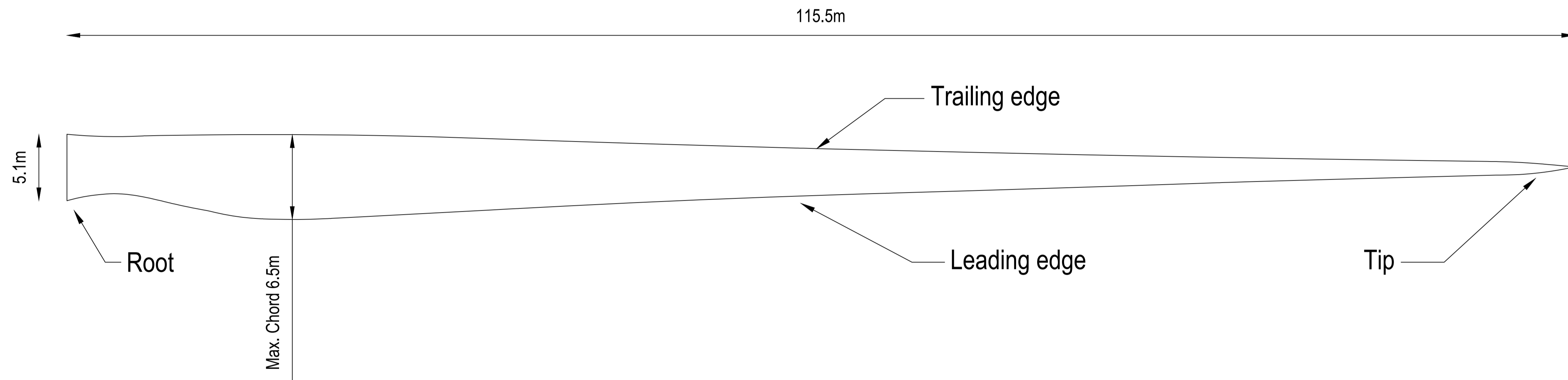
PLAN VIEW,1:200
